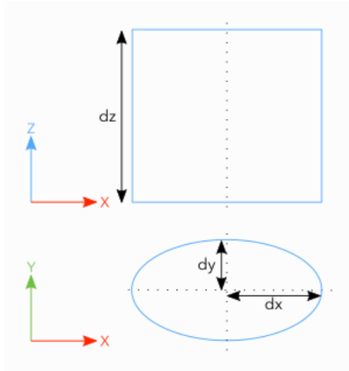
Figure 17: Elliptical tube parameters
