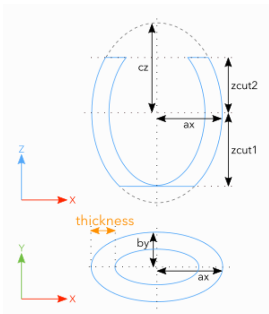
Figure 15: Ellipsoid parameters
