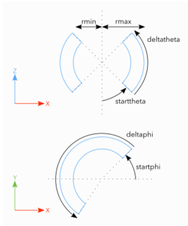
Figure 22: Sphere parameters
