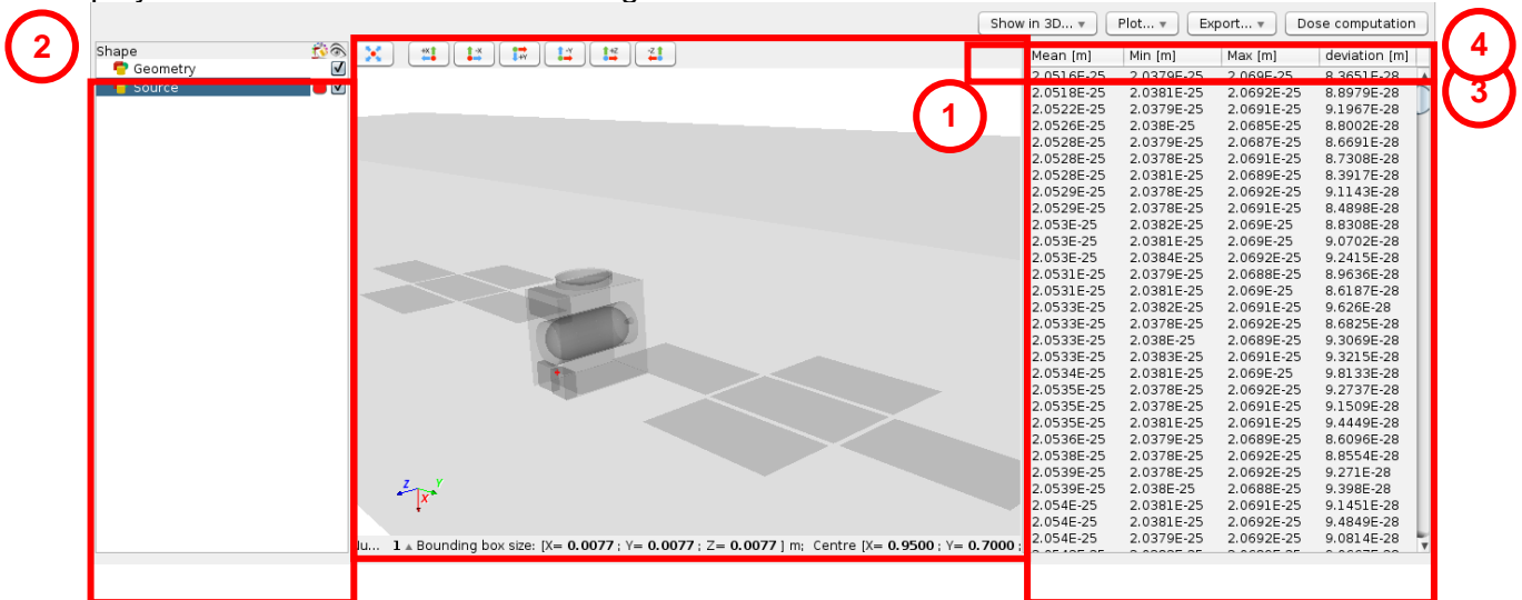
Figure 34: SSAM results
